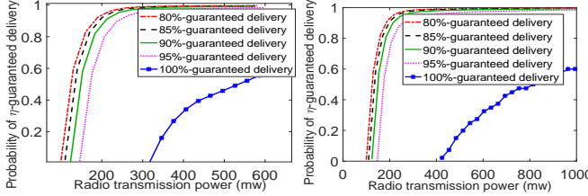
Fig. 6: Relationship between probability of \eta -guaranteed delivery and transmission power with interference and holes.
