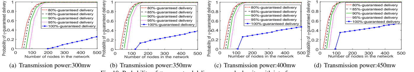
Fig. 10: Probability of \eta -guaranteed delivery vs. node density with interference.
