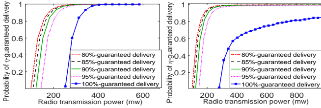
Fig. 4: Relationship between probability of \eta -guaranteed delivery and transmission power with interference.
