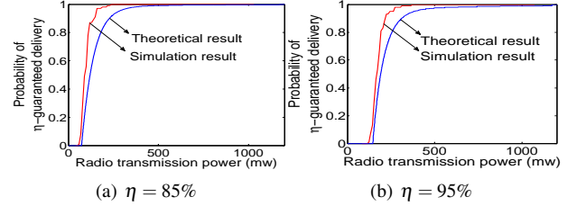
Fig. 15: Probability of \eta -guaranteed delivery vs. transmission power with holes (path-loss exponent \alpha = 3 , N = 200 , interval=2 seconds).
