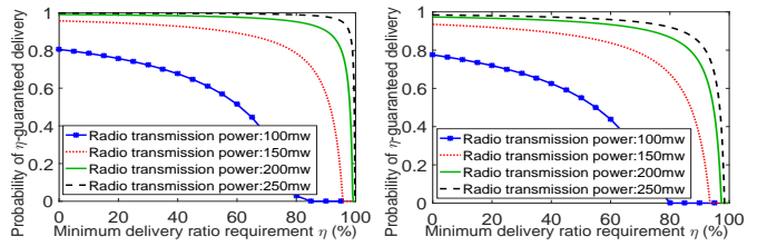
Fig. 5: Relationship between probability of \eta -guaranteed delivery and the minimum delivery ratio requirement \eta .
