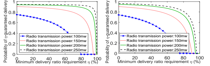
Fig. 7: Relationship between probability of \eta -guaranteed delivery and the minimum delivery ratio requirement \eta with hole consideration.
